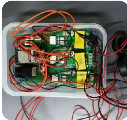
THREE-PHASE ENERGY METER (MFM)
