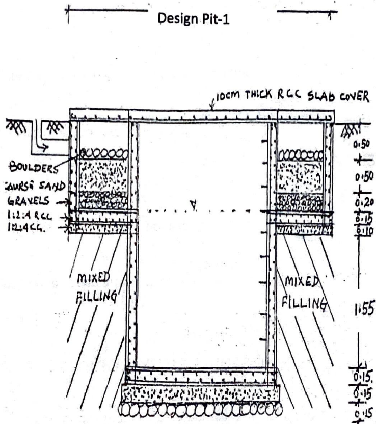
SECTION OF STORAGE TANK AND FILTER PLANT SCALE: 1 m = 2 cm
