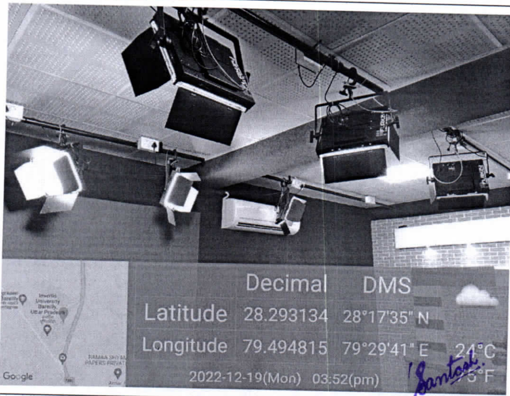
6 point Studio Lighting setup
